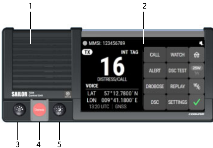
Figure 1: Controls on the front plate of the Control Unit
